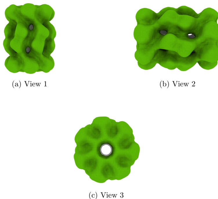
Figure 4: Isosurface at threshold=5.890000. Views generated by ChimeraX at a the following X, Y, Z angles: View 1 (0, -90, -90), View 2 (-90, 0, -90), View 3 (0, 0, 0).
