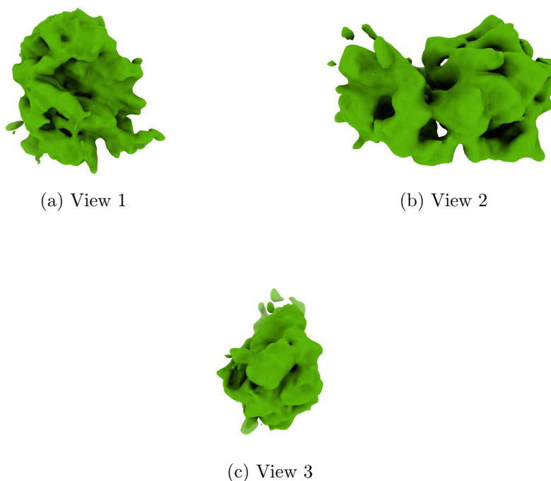
Figure 4: Isosurface at threshold=0.031100. Views generated by ChimeraX at a the following X, Y, Z angles: View 1 (0, -90, -90), View 2 (-90, 0, -90), View 3 (0, 0, 0).
