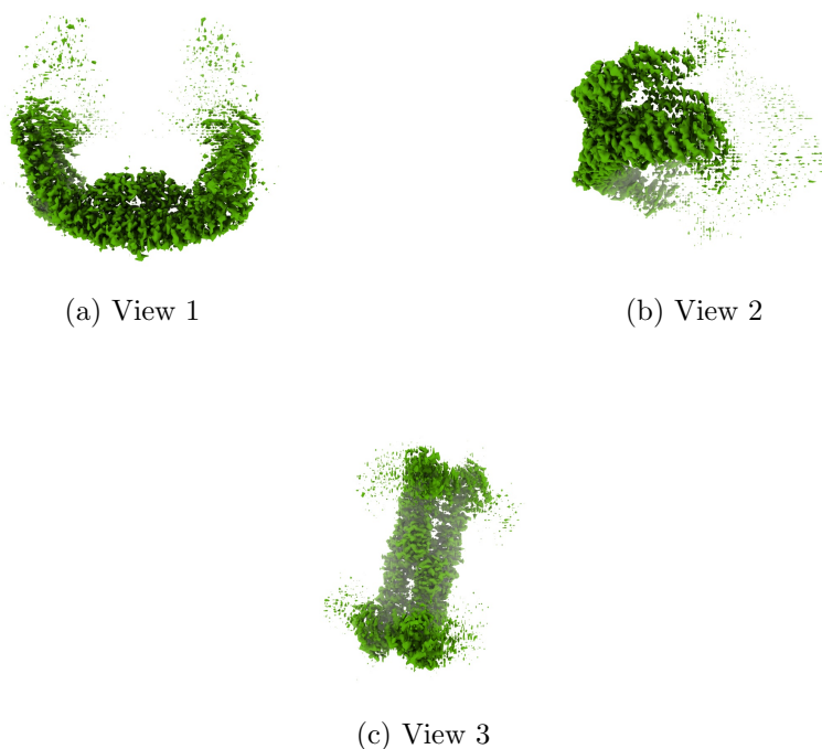
Figure 4: Isosurface at threshold=0.359000. Views generated by ChimeraX at a the following X, Y, Z angles: View 1 (0, -90, -90), View 2 (-90, 0, -90), View 3 (0, 0, 0).
