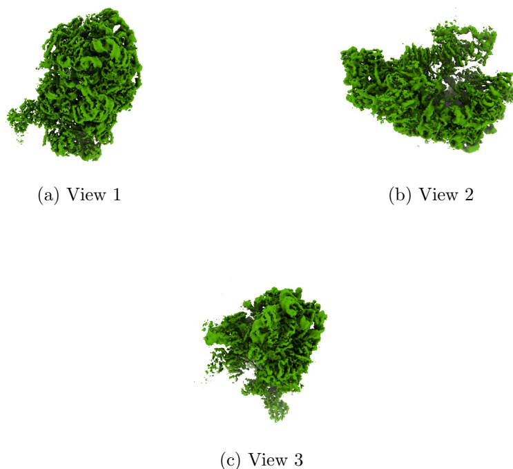
Figure 4: Isosurface at threshold=0.313000. Views generated by ChimeraX at a the following X, Y, Z angles: View 1 (0, -90, -90), View 2 (-90, 0, -90), View 3 (0, 0, 0).
