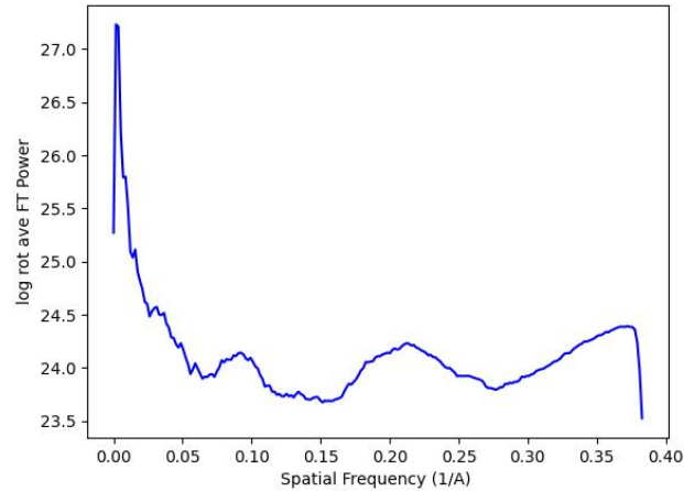
Figure 38: Logarithm of the radial average of the input map power in Fourier space.
