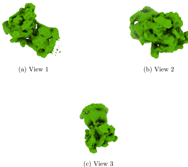
Figure 4: Isosurface at threshold=0.005800. Views generated by ChimeraX at a the following X, Y, Z angles: View 1 (0, -90, -90), View 2 (-90, 0, -90), View 3 (0, 0, 0).
