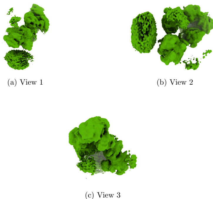
Figure 4: Isosurface at threshold=0.349000. Views generated by ChimeraX at a the following X, Y, Z angles: View 1 (0, -90, -90), View 2 (-90, 0, -90), View 3 (0, 0, 0).
