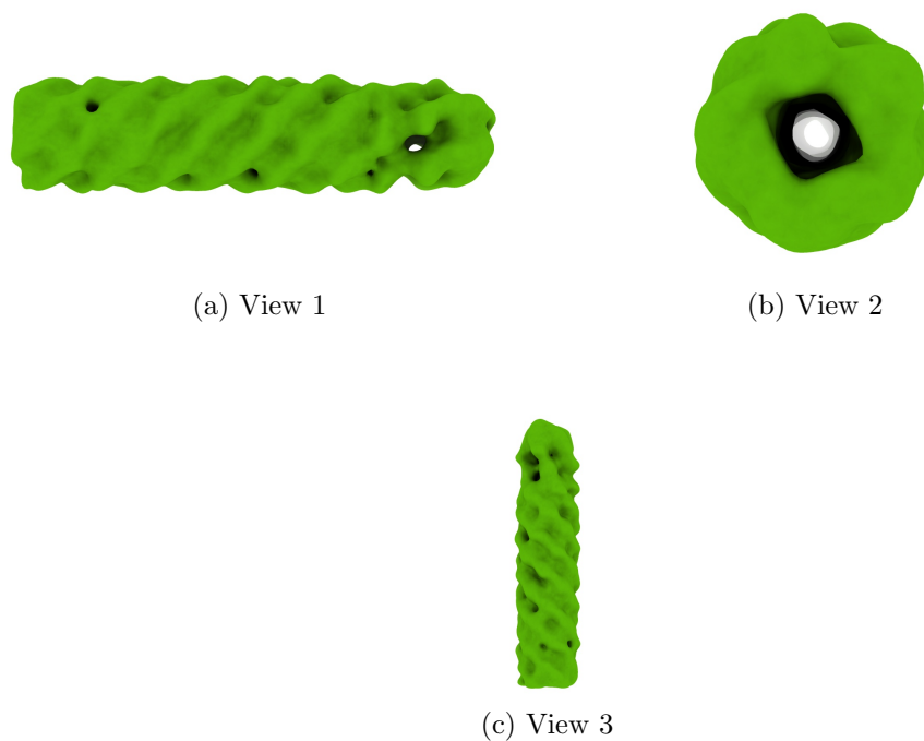
Figure 4: Isosurface at threshold=0.033200. Views generated by ChimeraX at a the following X, Y, Z angles: View 1 (0, -90, -90), View 2 (-90, 0, -90), View 3 (0, 0, 0).
