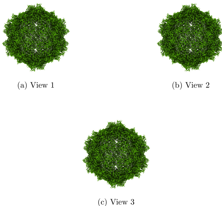
Figure 4: Isosurface at threshold=0.839000. Views generated by ChimeraX at a the following X, Y, Z angles: View 1 (0, -90, -90), View 2 (-90, 0, -90), View 3 (0, 0, 0).
