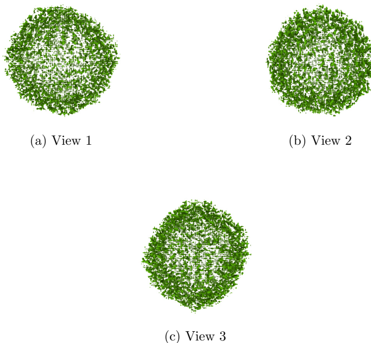
Figure 4: Isosurface at threshold=2.100000. Views generated by ChimeraX at a the following X, Y, Z angles: View 1 (0, -90, -90), View 2 (-90, 0, -90), View 3 (0, 0, 0).
