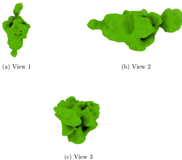
Figure 4: Isosurface at threshold=0.294000. Views generated by ChimeraX at a the following X, Y, Z angles: View 1 (0, -90, -90), View 2 (-90, 0, -90), View 3 (0, 0, 0).
