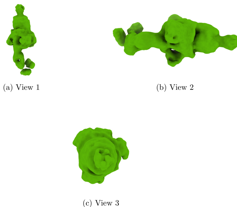
Figure 4: Isosurface at threshold=0.397000. Views generated by ChimeraX at a the following X, Y, Z angles: View 1 (0, -90, -90), View 2 (-90, 0, -90), View 3 (0, 0, 0).
