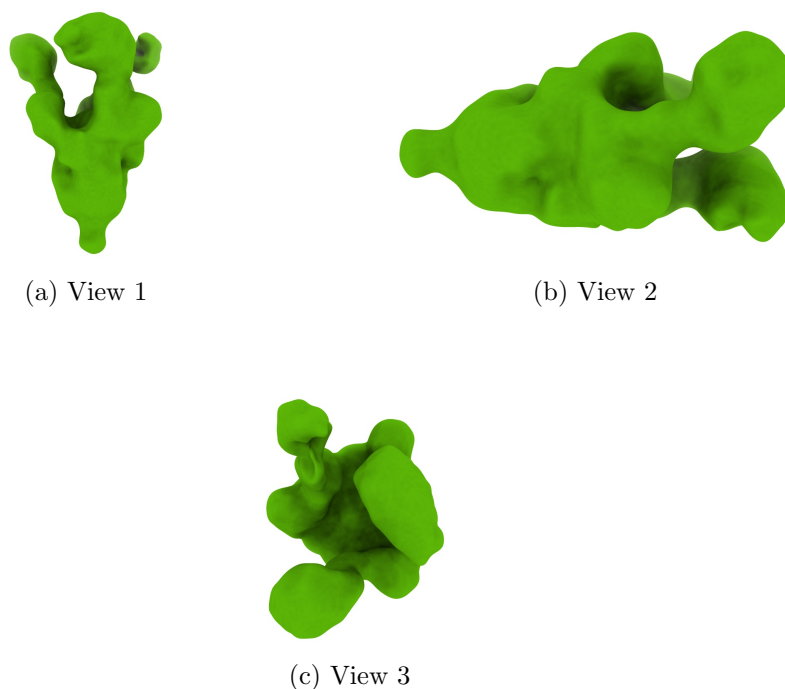
Figure 4: Isosurface at threshold=0.391000. Views generated by ChimeraX at a the following X, Y, Z angles: View 1 (0, -90, -90), View 2 (-90, 0, -90), View 3 (0, 0, 0).
