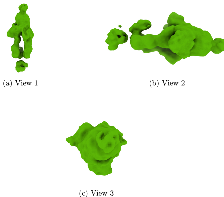
Figure 4: Isosurface at threshold=1.230000. Views generated by ChimeraX at a the following X, Y, Z angles: View 1 (0, -90, -90), View 2 (-90, 0, -90), View 3 (0, 0, 0).
