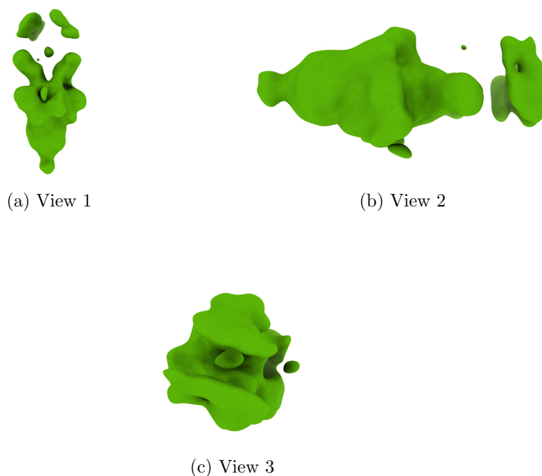
Figure 4: Isosurface at threshold=0.161000. Views generated by ChimeraX at a the following X, Y, Z angles: View 1 (0, -90, -90), View 2 (-90, 0, -90), View 3 (0, 0, 0).
