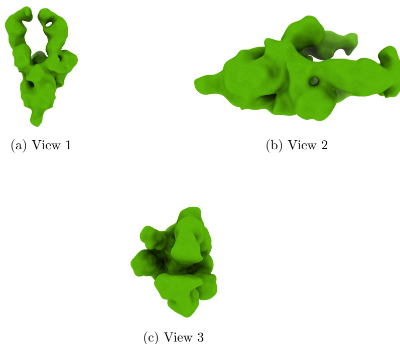
Figure 4: Isosurface at threshold=0.272000. Views generated by ChimeraX at a the following X, Y, Z angles: View 1 (0, -90, -90), View 2 (-90, 0, -90), View 3 (0, 0, 0).
