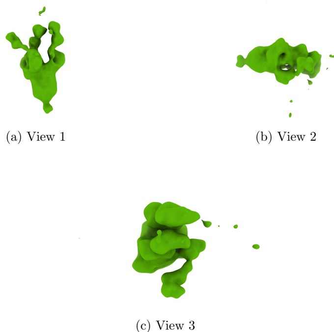
Figure 4: Isosurface at threshold=0.095900. Views generated by ChimeraX at a the following X, Y, Z angles: View 1 (0, -90, -90), View 2 (-90, 0, -90), View 3 (0, 0, 0).
