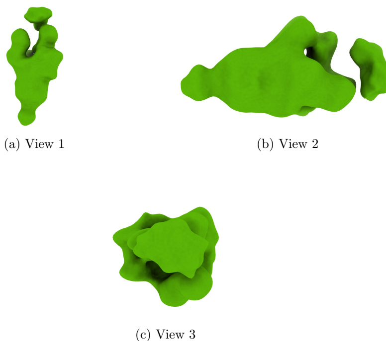
Figure 4: Isosurface at threshold=0.643000. Views generated by ChimeraX at a the following X, Y, Z angles: View 1 (0, -90, -90), View 2 (-90, 0, -90), View 3 (0, 0, 0).
