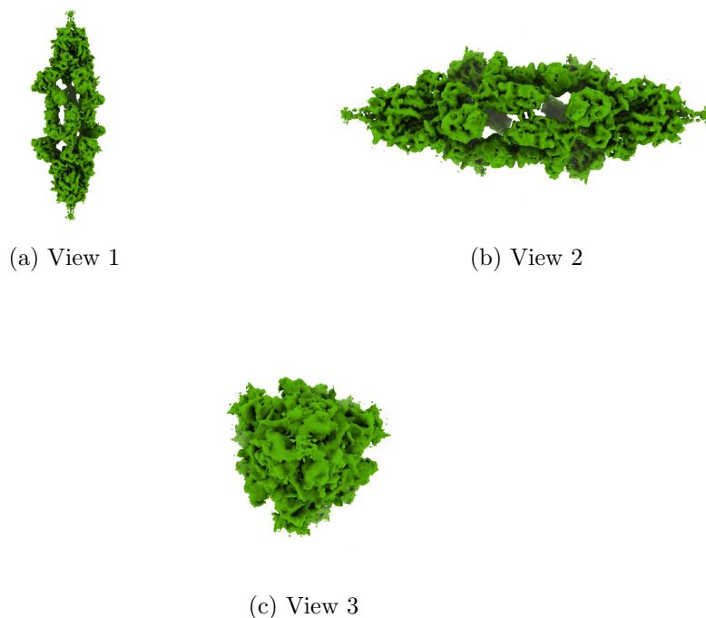
Figure 4: Isosurface at threshold=0.240000. Views generated by ChimeraX at a the following X, Y, Z angles: View 1 (0, -90, -90), View 2 (-90, 0, -90), View 3 (0, 0, 0).
