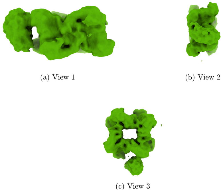
Figure 4: Isosurface at threshold=0.009890. Views generated by ChimeraX at a the following X, Y, Z angles: View 1 (0, -90, -90), View 2 (-90, 0, -90), View 3 (0, 0, 0).
