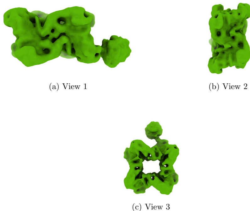
Figure 4: Isosurface at threshold=0.016200. Views generated by ChimeraX at a the following X, Y, Z angles: View 1 (0, -90, -90), View 2 (-90, 0, -90), View 3 (0, 0, 0).
