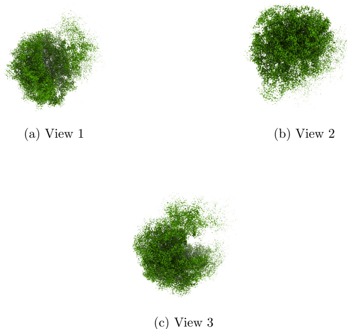
Figure 4: Isosurface at threshold=0.061400. Views generated by ChimeraX at a the following X, Y, Z angles: View 1 (0, -90, -90), View 2 (-90, 0, -90), View 3 (0, 0, 0).
