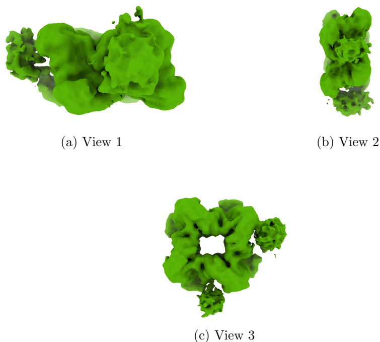
Figure 4: Isosurface at threshold=0.008050. Views generated by ChimeraX at a the following X, Y, Z angles: View 1 (0, -90, -90), View 2 (-90, 0, -90), View 3 (0, 0, 0).
