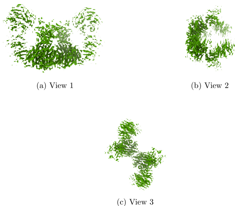
Figure 4: Isosurface at threshold=0.700000. Views generated by ChimeraX at a the following X, Y, Z angles: View 1 (0, -90, -90), View 2 (-90, 0, -90), View 3 (0, 0, 0).
