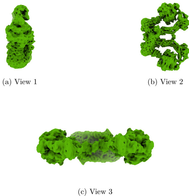
Figure 4: Isosurface at threshold=0.070000. Views generated by ChimeraX at a the following X, Y, Z angles: View 1 (0, -90, -90), View 2 (-90, 0, -90), View 3 (0, 0, 0).
