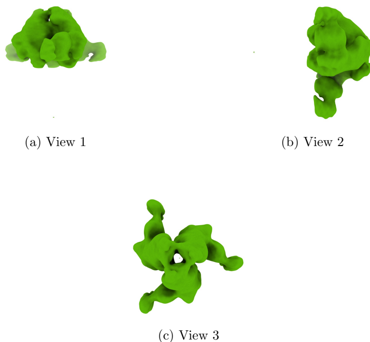
Figure 4: Isosurface at threshold=0.720000. Views generated by ChimeraX at a the following X, Y, Z angles: View 1 (0, -90, -90), View 2 (-90, 0, -90), View 3 (0, 0, 0).
