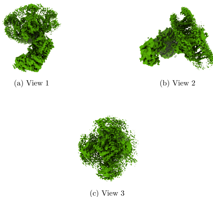
Figure 4: Isosurface at threshold=0.002600. Views generated by ChimeraX at a the following X, Y, Z angles: View 1 (0, -90, -90), View 2 (-90, 0, -90), View 3 (0, 0, 0).
