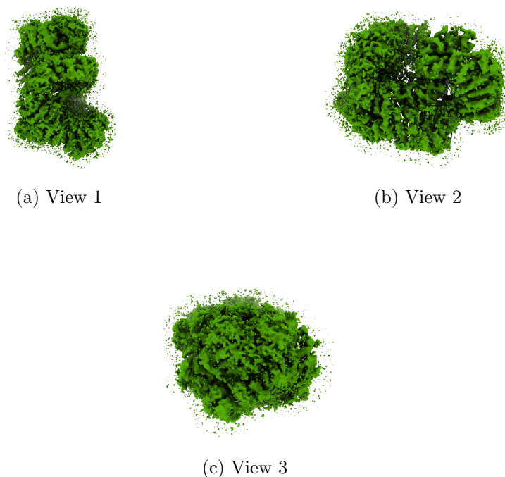
Figure 4: Isosurface at threshold=0.300000. Views generated by ChimeraX at a the following X, Y, Z angles: View 1 (0, -90, -90), View 2 (-90, 0, -90), View 3 (0, 0, 0).
