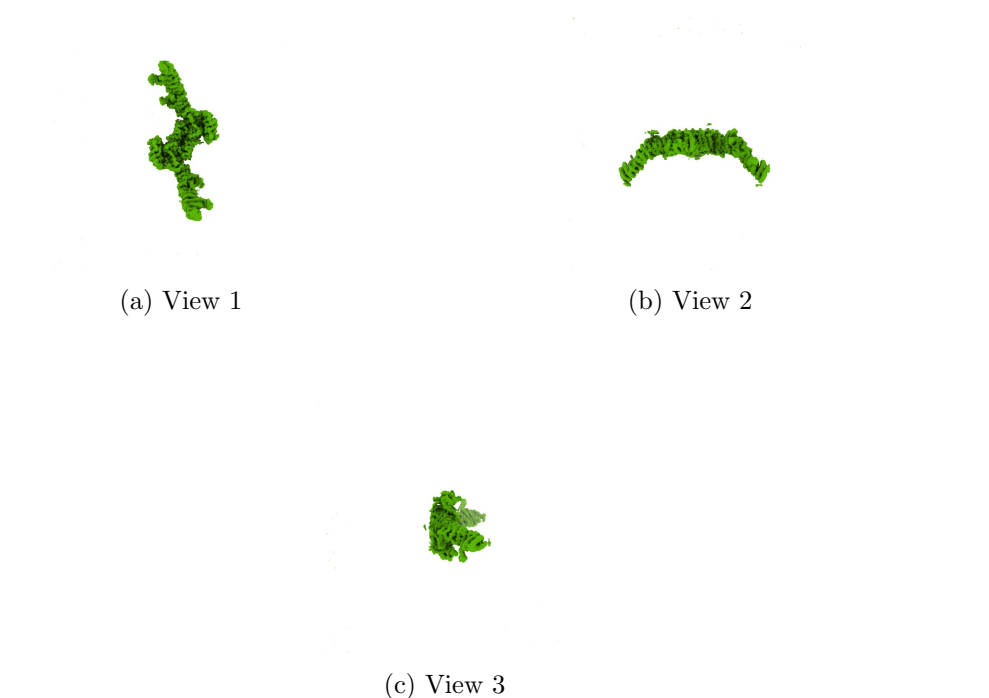
Figure 4: Isosurface at threshold=0.010000. Views generated by ChimeraX at a the following X, Y, Z angles: View 1 (0, -90, -90), View 2 (-90, 0, -90), View 3 (0, 0, 0).
