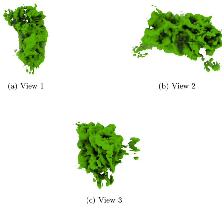
Figure 4: Isosurface at threshold=0.607000. Views generated by ChimeraX at a the following X, Y, Z angles: View 1 (0, -90, -90), View 2 (-90, 0, -90), View 3 (0, 0, 0).
