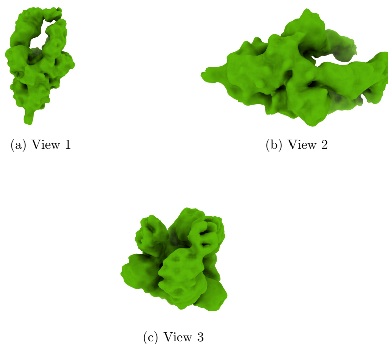
Figure 4: Isosurface at threshold=0.300000. Views generated by ChimeraX at a the following X, Y, Z angles: View 1 (0, -90, -90), View 2 (-90, 0, -90), View 3 (0, 0, 0).
