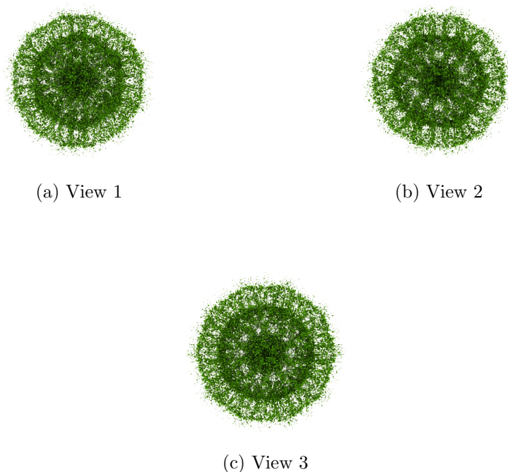
Figure 4: Isosurface at threshold=5.500000. Views generated by ChimeraX at a the following X, Y, Z angles: View 1 (0, -90, -90), View 2 (-90, 0, -90), View 3 (0, 0, 0).
