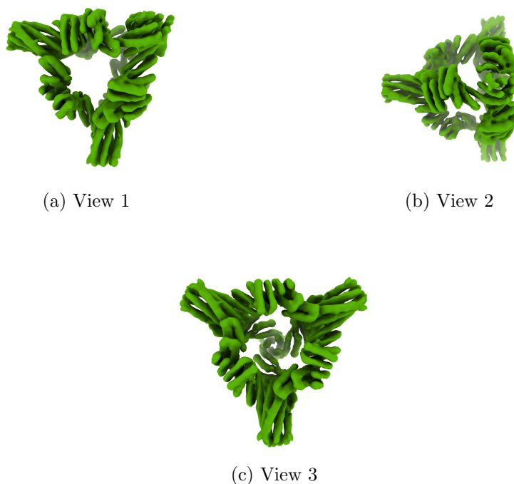
Figure 4: Isosurface at threshold=0.161000. Views generated by ChimeraX at a the following X, Y, Z angles: View 1 (0, -90, -90), View 2 (-90, 0, -90), View 3 (0, 0, 0).
