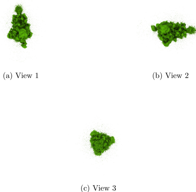
Figure 4: Isosurface at threshold=0.060100. Views generated by ChimeraX at a the following X, Y, Z angles: View 1 (0, -90, -90), View 2 (-90, 0, -90), View 3 (0, 0, 0).
