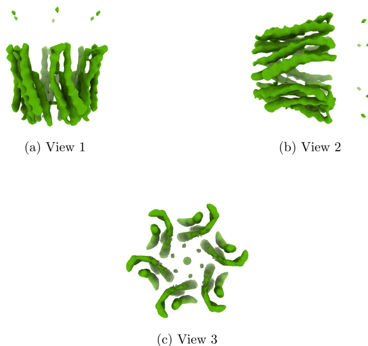
Figure 4: Isosurface at threshold=0.469000. Views generated by ChimeraX at a the following X, Y, Z angles: View 1 (0, -90, -90), View 2 (-90, 0, -90), View 3 (0, 0, 0).
