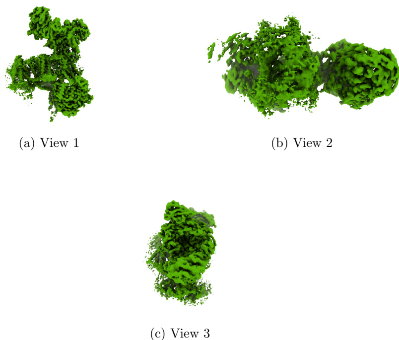
Figure 4: Isosurface at threshold=0.003300. Views generated by ChimeraX at a the following X, Y, Z angles: View 1 (0, -90, -90), View 2 (-90, 0, -90), View 3 (0, 0, 0).
