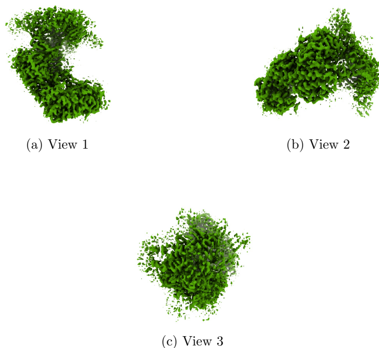
Figure 4: Isosurface at threshold=0.005900. Views generated by ChimeraX at a the following X, Y, Z angles: View 1 (0, -90, -90), View 2 (-90, 0, -90), View 3 (0, 0, 0).
