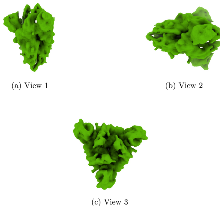
Figure 4: Isosurface at threshold=0.046100. Views generated by ChimeraX at a the following X, Y, Z angles: View 1 (0, -90, -90), View 2 (-90, 0, -90), View 3 (0, 0, 0).
