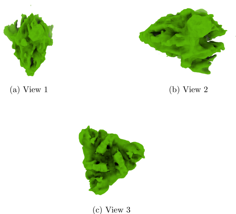
Figure 4: Isosurface at threshold=0.033200. Views generated by ChimeraX at a the following X, Y, Z angles: View 1 (0, -90, -90), View 2 (-90, 0, -90), View 3 (0, 0, 0).
