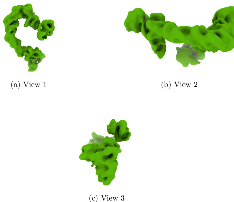
Figure 4: Isosurface at threshold=0.174000. Views generated by ChimeraX at a the following X, Y, Z angles: View 1 (0, -90, -90), View 2 (-90, 0, -90), View 3 (0, 0, 0).
