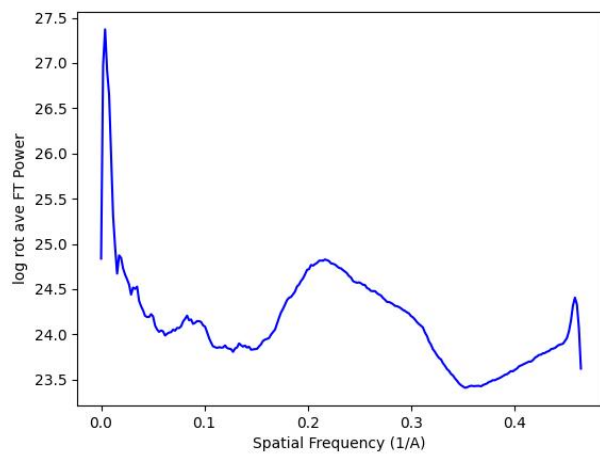
Figure 33: Logarithm of the radial average of the input map power in Fourier space.
