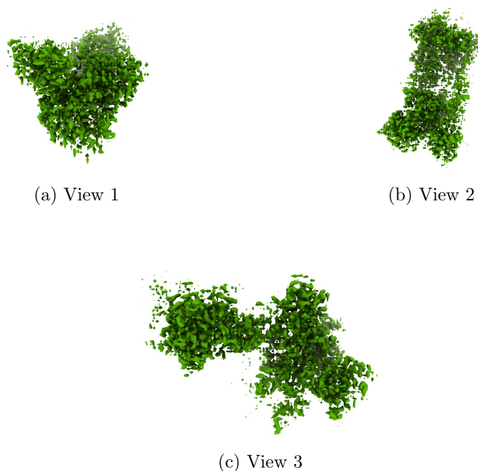
Figure 4: Isosurface at threshold=0.650000. Views generated by ChimeraX at a the following X, Y, Z angles: View 1 (0, -90, -90), View 2 (-90, 0, -90), View 3 (0, 0, 0).
