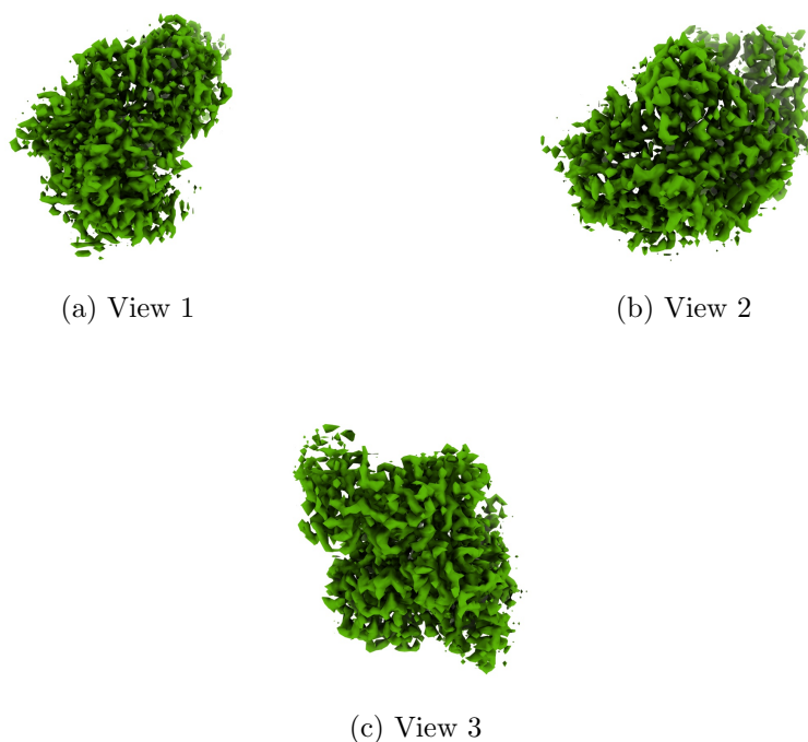
Figure 4: Isosurface at threshold=0.888000. Views generated by ChimeraX at a the following X, Y, Z angles: View 1 (0, -90, -90), View 2 (-90, 0, -90), View 3 (0, 0, 0).
