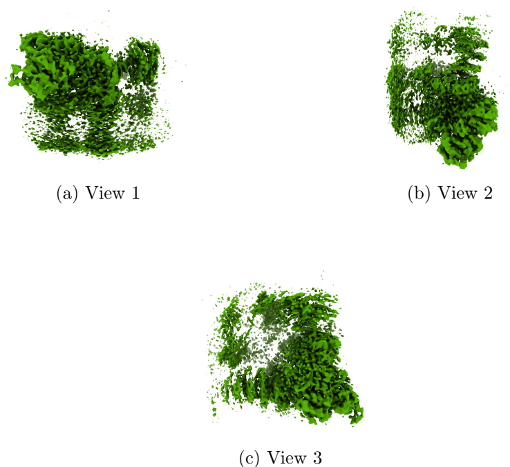
Figure 4: Isosurface at threshold=0.328000. Views generated by ChimeraX at a the following X, Y, Z angles: View 1 (0, -90, -90), View 2 (-90, 0, -90), View 3 (0, 0, 0).
