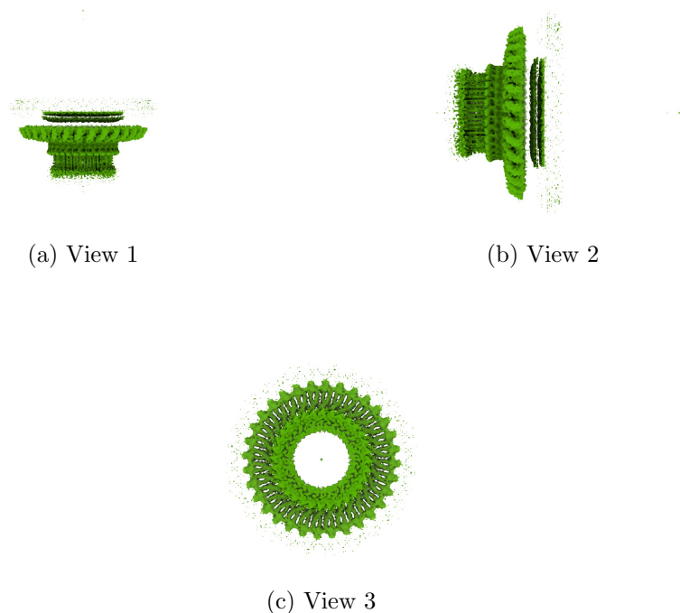
Figure 4: Isosurface at threshold=0.237000. Views generated by ChimeraX at a the following X, Y, Z angles: View 1 (0, -90, -90), View 2 (-90, 0, -90), View 3 (0, 0, 0).
