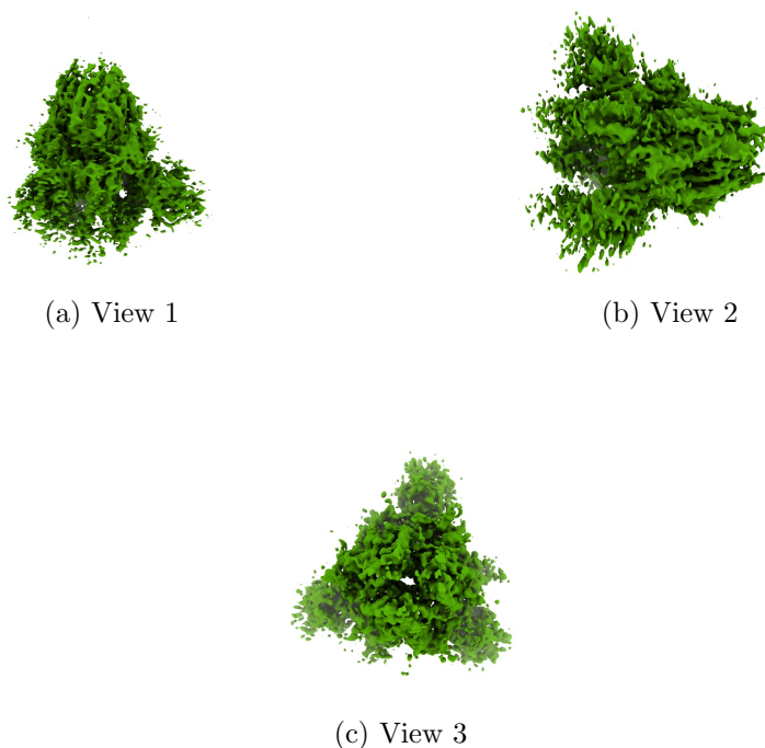
Figure 4: Isosurface at threshold=0.143000. Views generated by ChimeraX at a the following X, Y, Z angles: View 1 (0, -90, -90), View 2 (-90, 0, -90), View 3 (0, 0, 0).
