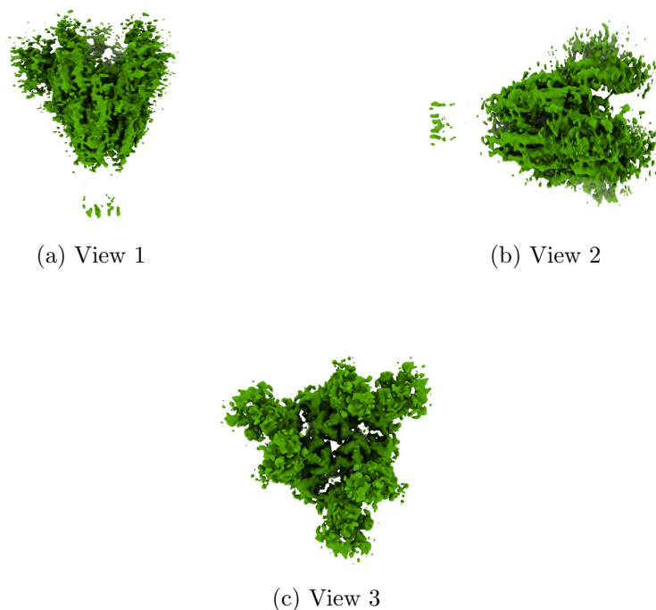
Figure 4: Isosurface at threshold=0.133000. Views generated by ChimeraX at a the following X, Y, Z angles: View 1 (0, -90, -90), View 2 (-90, 0, -90), View 3 (0, 0, 0).
