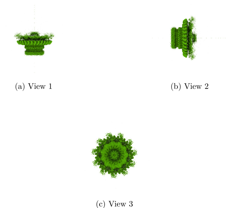
Figure 4: Isosurface at threshold=0.148000. Views generated by ChimeraX at a the following X, Y, Z angles: View 1 (0, -90, -90), View 2 (-90, 0, -90), View 3 (0, 0, 0).
