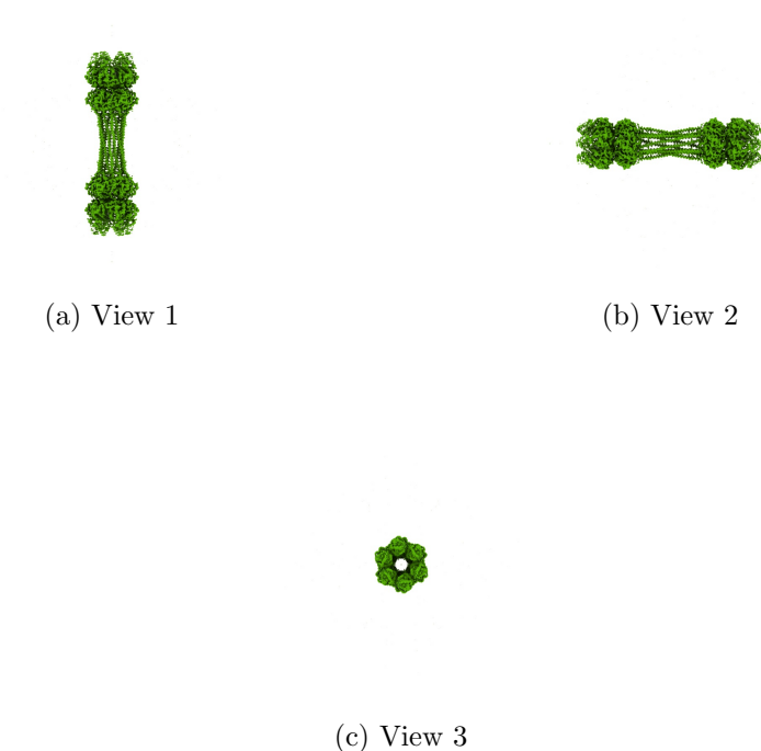
Figure 4: Isosurface at threshold=0.180000. Views generated by ChimeraX at a the following X, Y, Z angles: View 1 (0, -90, -90), View 2 (-90, 0, -90), View 3 (0, 0, 0).
