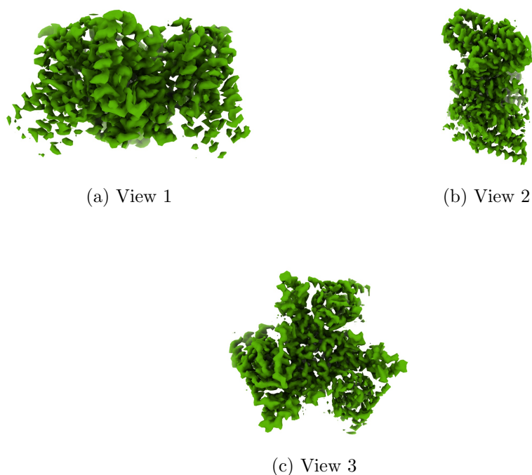
Figure 4: Isosurface at threshold=0.401000. Views generated by ChimeraX at a the following X, Y, Z angles: View 1 (0, -90, -90), View 2 (-90, 0, -90), View 3 (0, 0, 0).
