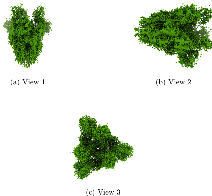
Figure 4: Isosurface at threshold=0.001500. Views generated by ChimeraX at a the following X, Y, Z angles: View 1 (0, -90, -90), View 2 (-90, 0, -90), View 3 (0, 0, 0).
